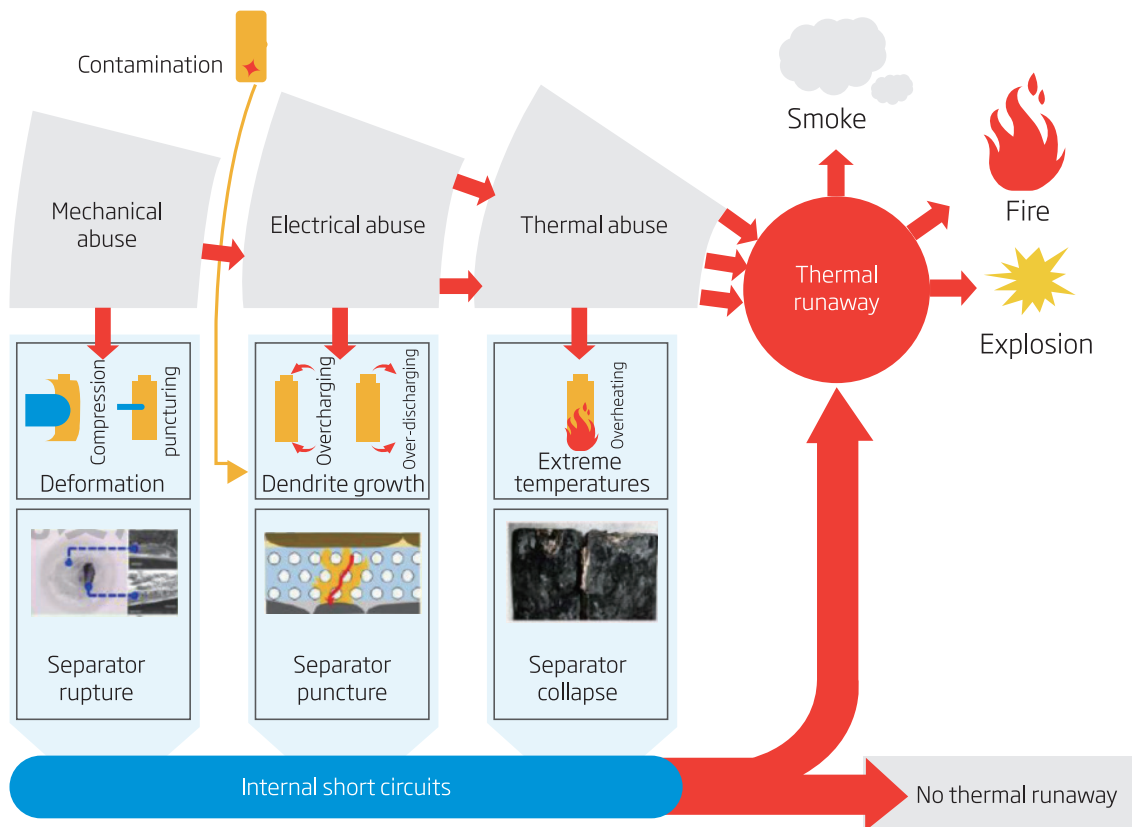
Image credit: Feng X. et al. Mechanisms of Thermal Runaway in Lithium-Ion Batteries for Electric Vehicles: A Review, Energy Storage Materials, 2018, 10: 246-267
