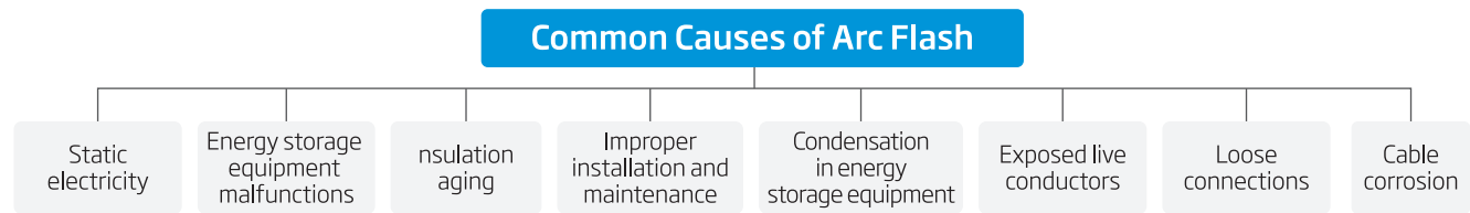
Figure 8 Common Causes of Arc Flash
