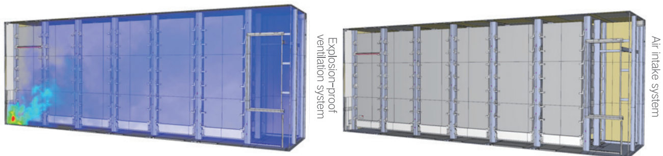
Figure 19 Combustible Gas Concentration in the Cabinet Minutes after Mechanical Exhaust System Activation
