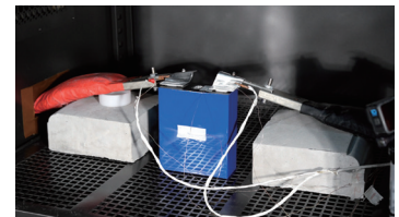
Short circuit performance test
