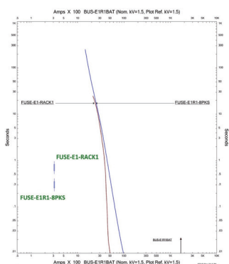
Figure 10 Short-Circuit Matching of Upper and Lower Level Fuses
