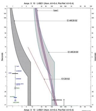
Figure 9 Matching of Different Circuit Breakers and Fuses
