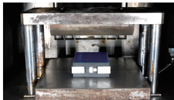
Crush performance test
