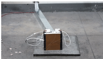
Overcharge thermal runaway performance test
