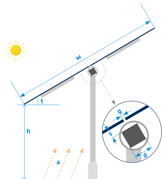
Figure 29. Main parameters affecting the Structure Shading Factor (SSF)
