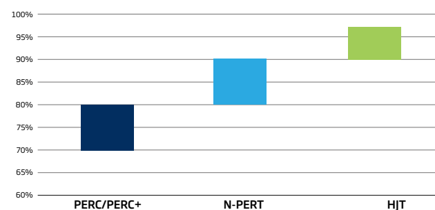
Figure 6. Bifaciality by different cell technologies
