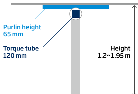
Figure 13. Selected 1P tracker main design parameters
